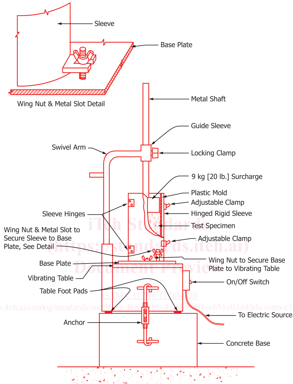
FIG. 1 Vibrating Table—Cylinder Preparation (Type B Mold)
