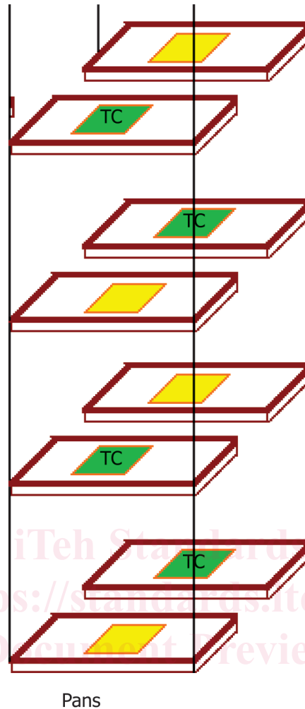
FIG. 32 Full Size Combination Oven Pan Thermocouple Placement
