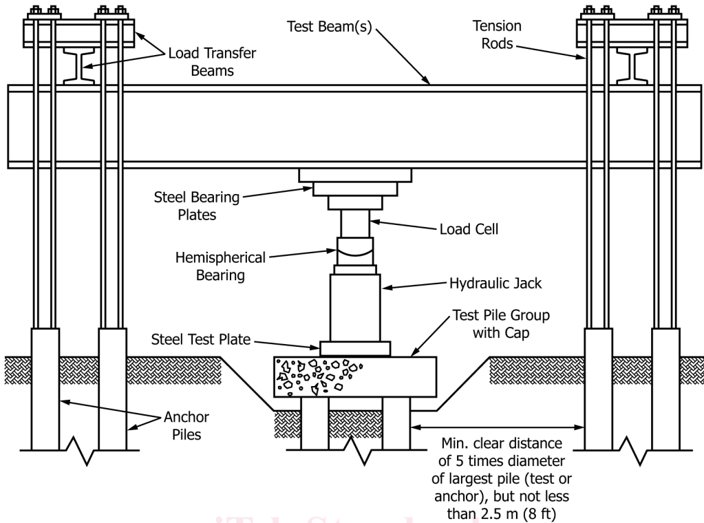
FIG. 2 Schematic of Hydraulic Jack on a Pile Element Group Acting Against an Anchored Reaction Frame
