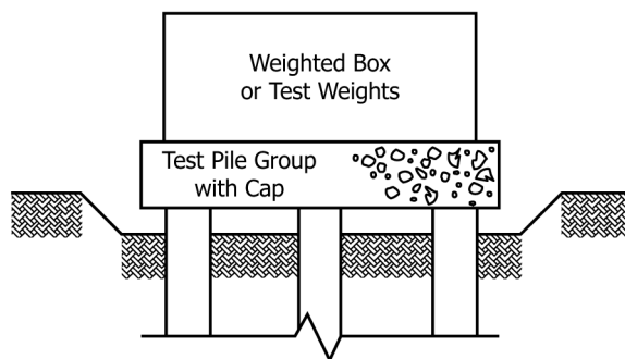
FIG. 4 Schematic of Direct Loading on a Single Pile Using Weighted Platform Element Group
