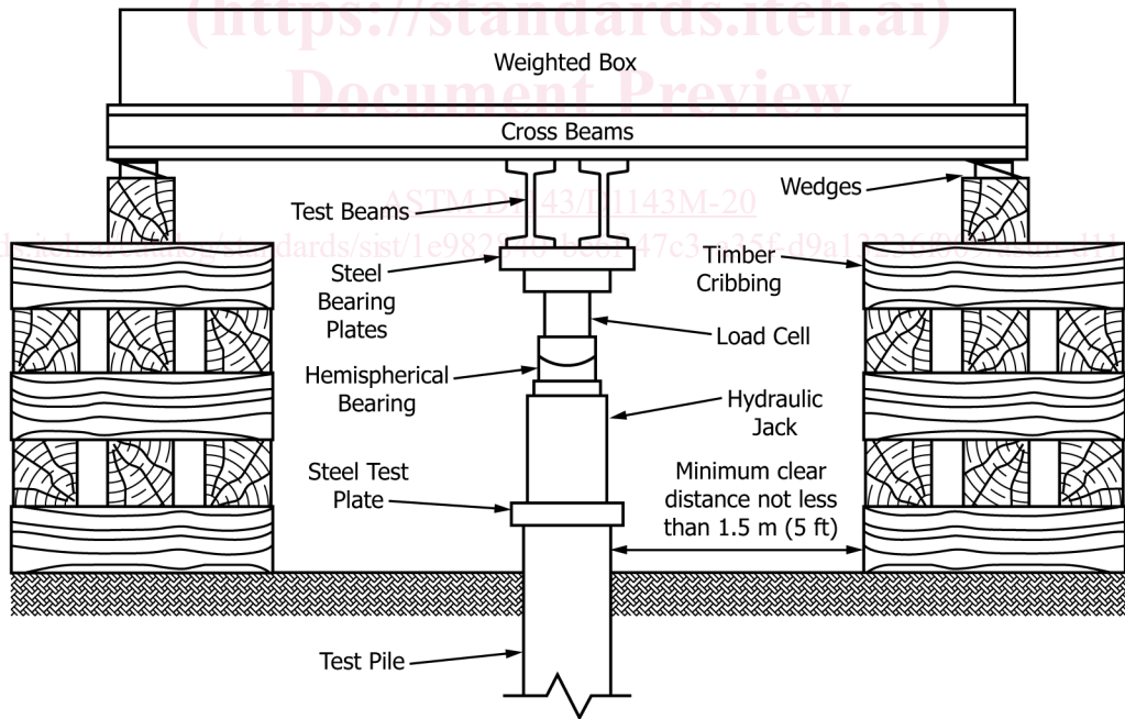
FIG. 3 Schematic Hydraulic Jack Acting Against on an Element Acting against a Weighted Box or Platform
