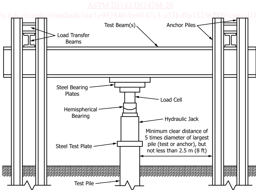
FIG. 1 Schematic of Hydraulic Jack Acting Against an Element Acting against Anchored Reaction Frame
