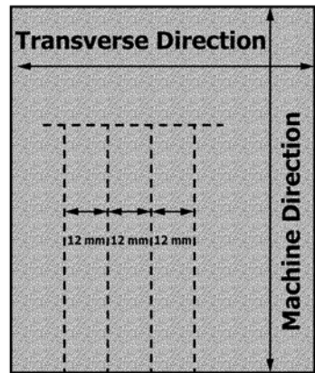
FIG. 2 Typical Sample of a Pressure Sensitive Article (Schematic for Sample Preparation)
