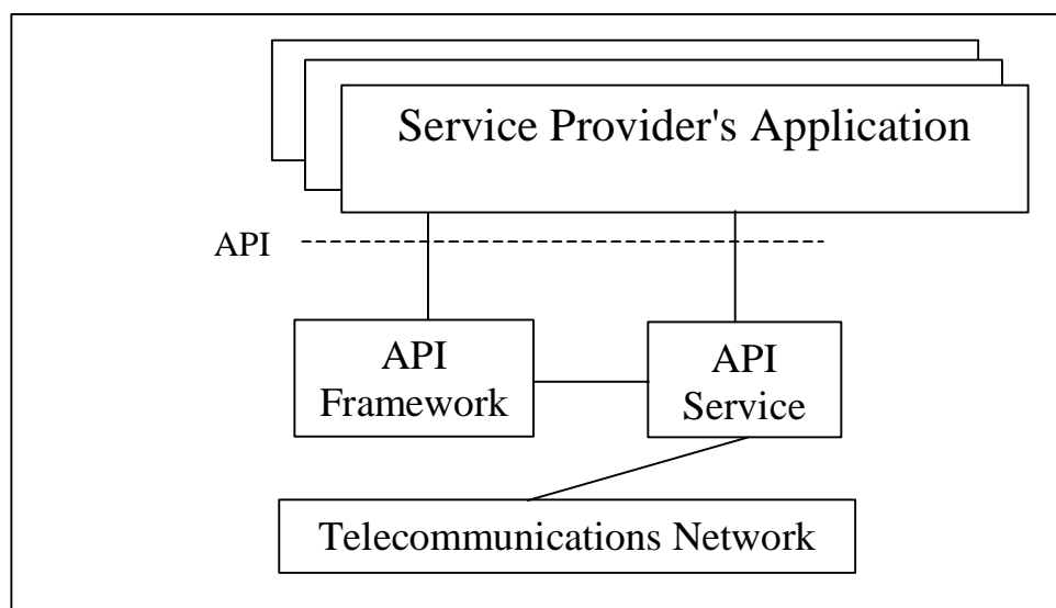
Figure 1: API Architecture
