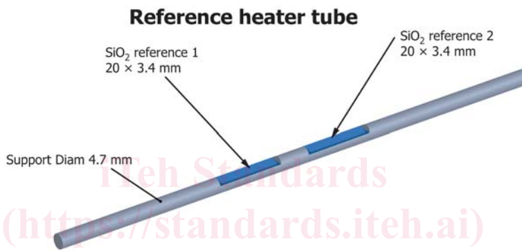
FIG. A2.2 Reference Heater Tube
