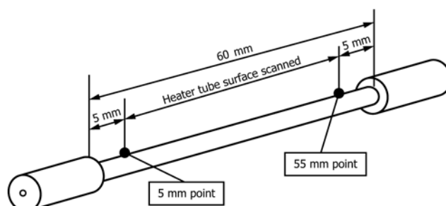
FIG. A2.7 Description of Heater Tube Scanned Surface
