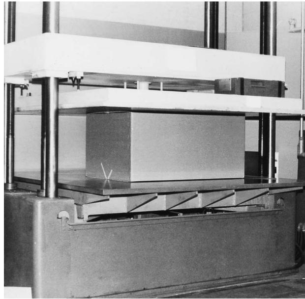
FIG. 1 Compression Applied Diagonally Opposite Edges Box Compression Top to Bottom Using a Fixed-Platen Machine
