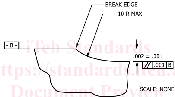
FIG. 9 Support Fixture—Details A and B (Inch-Pound Version)
