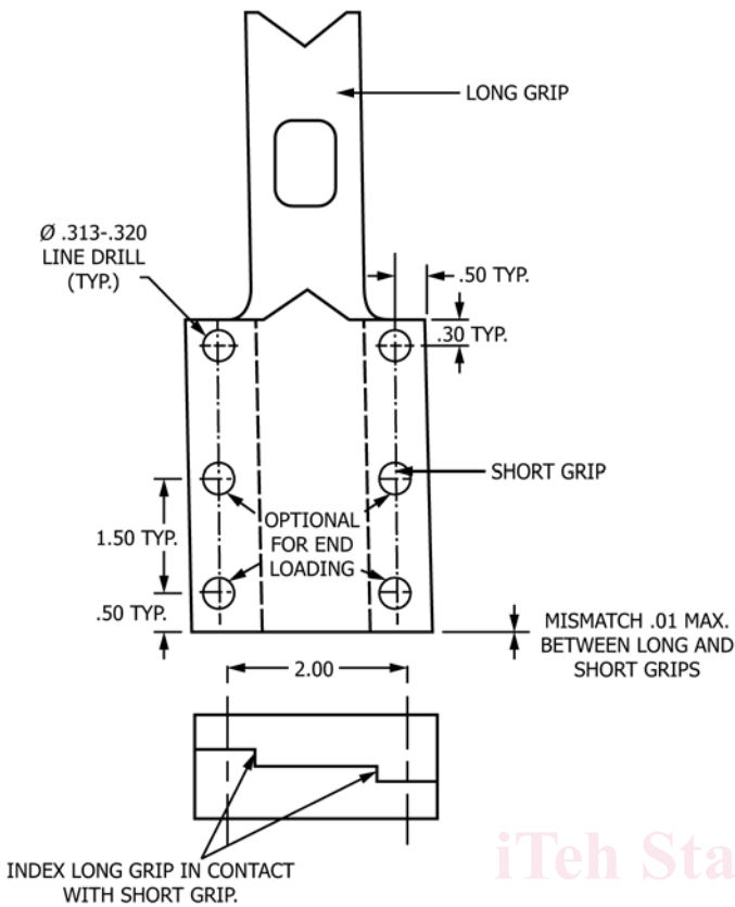
FIG. 3 Support Fixture—Line Drilling Details (Inch-Pound Version) NOTE 1— (a) All dimensions in inches. (b) The long grip and short grip should be part marked with a unique test fixture assembly identification. (c) Tolerance except as noted is linear \pm 0.01 in.
