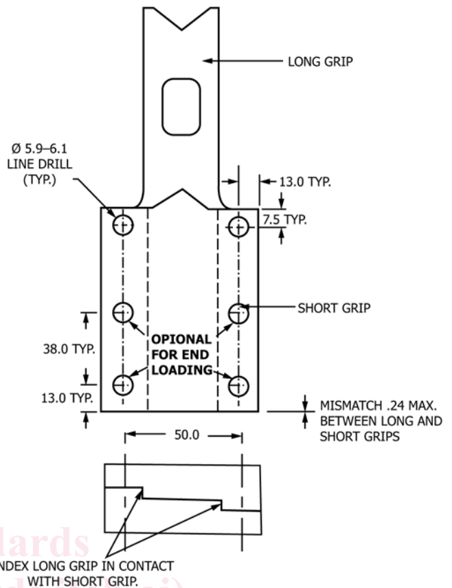
FIG. 4 Support Fixture—Line Drilling Details (SI Version) NOTE 1— (a) All dimensions in mm. (b) The long grip and short grip should be part marked with a unique test fixture assembly identification. (c) Tolerance except as noted is linear \pm 0.24 mm.
