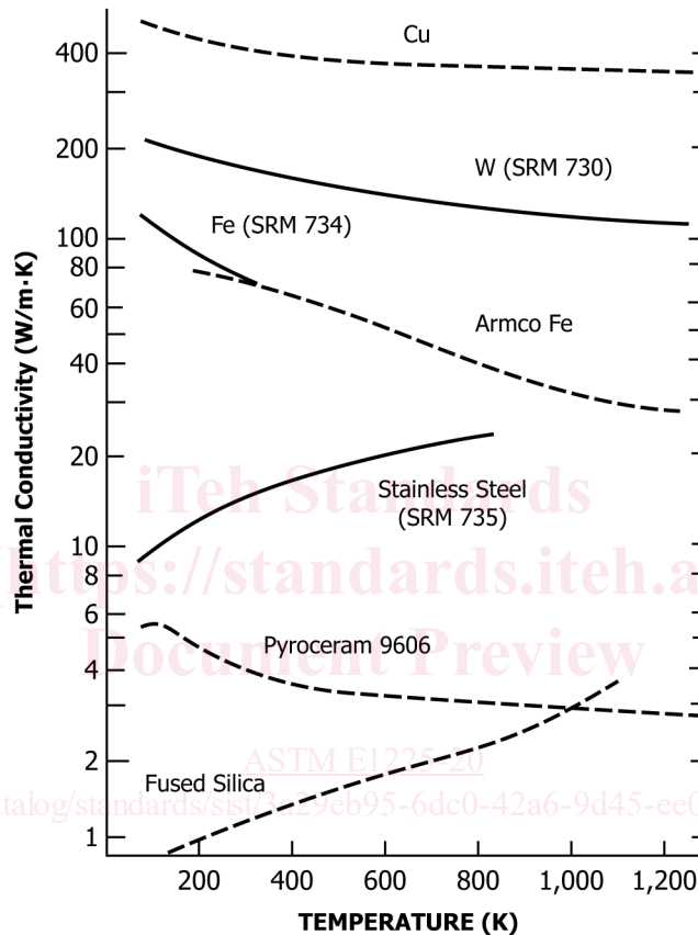
FIG. 2 Approximate Values for the Thermal Conductivity of Several Possible Recommended Reference Materials for Meter Bars
