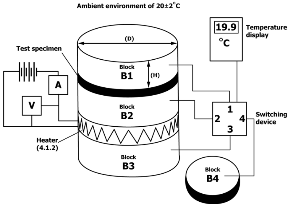
FIG. 1 SATRA Lees' Disc Thermal Conductivity Apparatus
