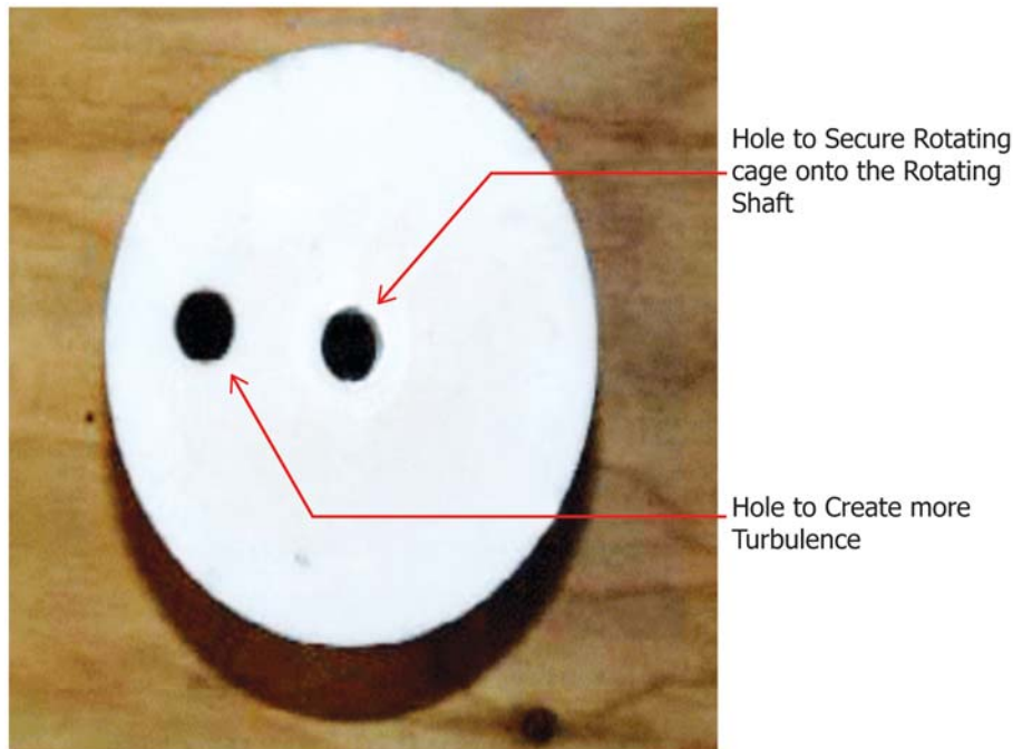
FIG. 3 Photo of Rotating Cage (Top View)
