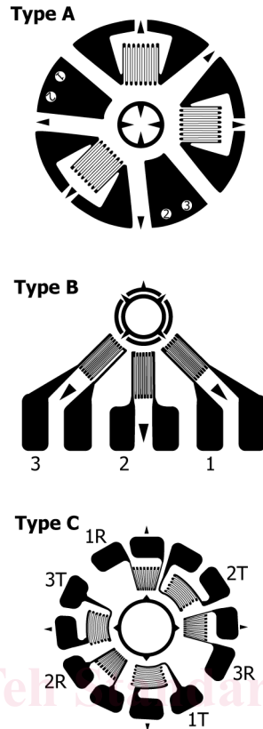
FIG. 42 Hole-Drilling Rosettes
