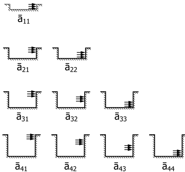
FIG. 34 Physical Interpretation of Coefficients a_{jk}
