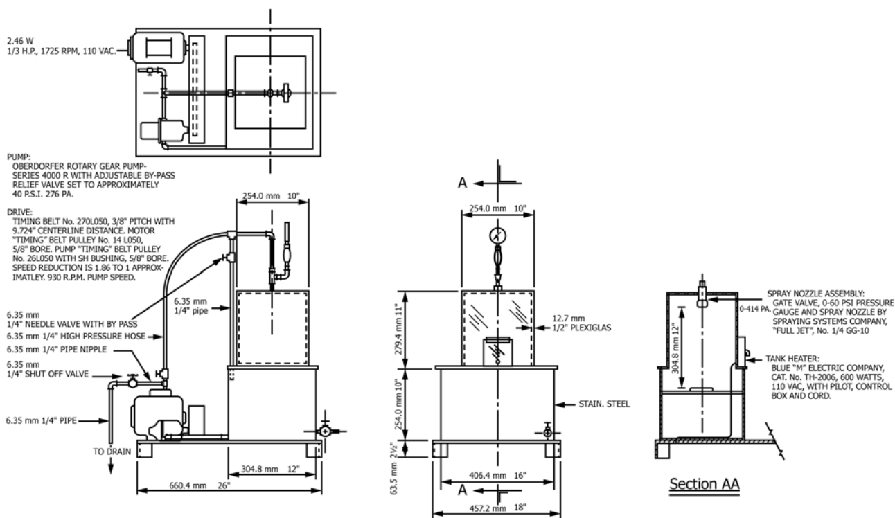
NOTE 1—The bypass valve shall be ahead of the gauge, not between the gauge and nozzle.
