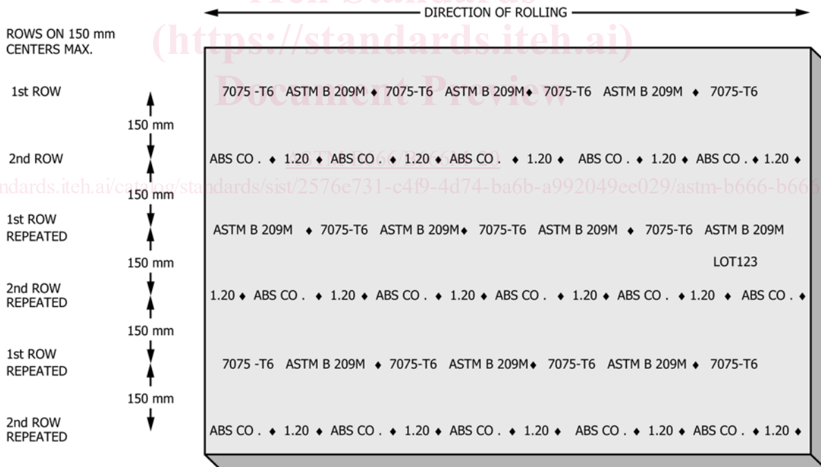
FIG. 4 Continuous Marking for Plate Through 0.375 in. and Flat Sheet 0.012 in. and Over (for O Temper, 0.020 in. and over) in Thickness, 6 Through 60 Inches in Width, and 36 Through 200 Inches in Length
