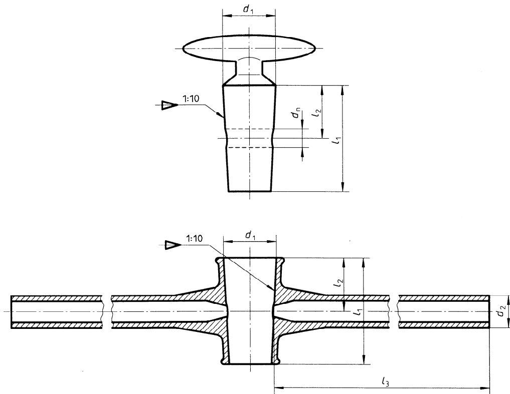
Figure 1 — Straight-bore stopcock, general appearance (standards.iteh.ai)
