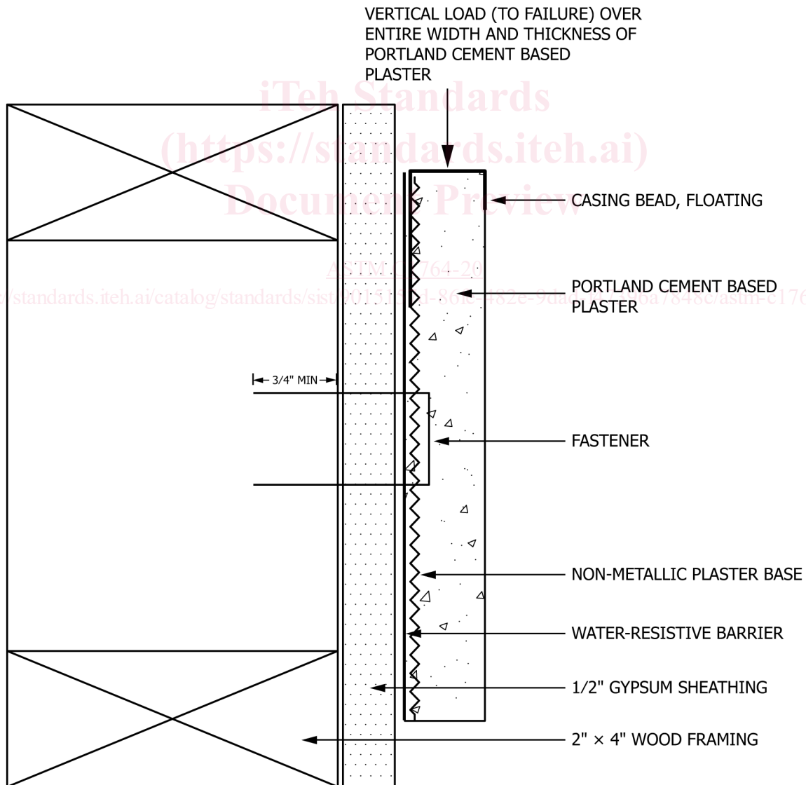
FIG. 1 Test Assembly
