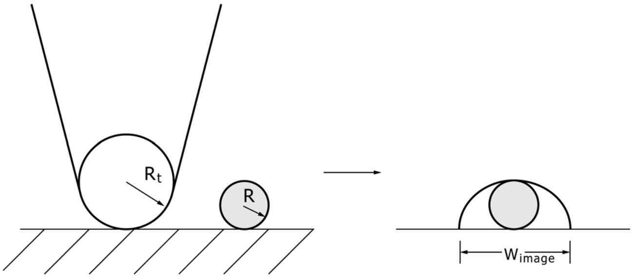
FIG. 8 Schematic of Tip Broadening Effect for an Idealized Spherical Tip (Radius R_t ) and Spherical Surface Feature (Radius R_s )
