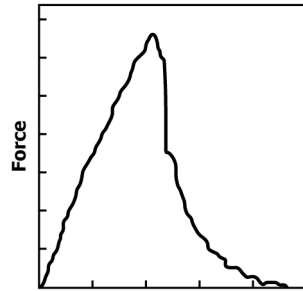
b) Pop-in Behavior - stable
