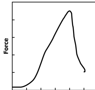
c) Stable Crack Extension
