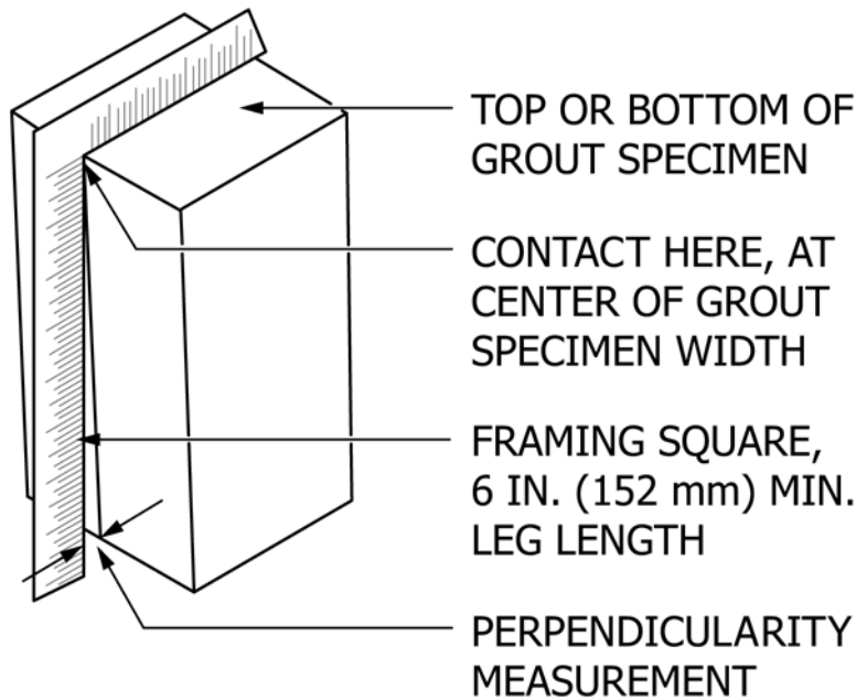
FIG. 5 Perpendicularity Measurement
