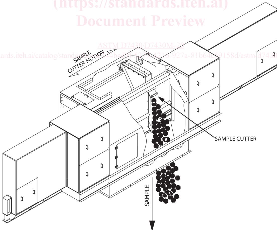
FIG. 2 Falling-Stream Sampler
