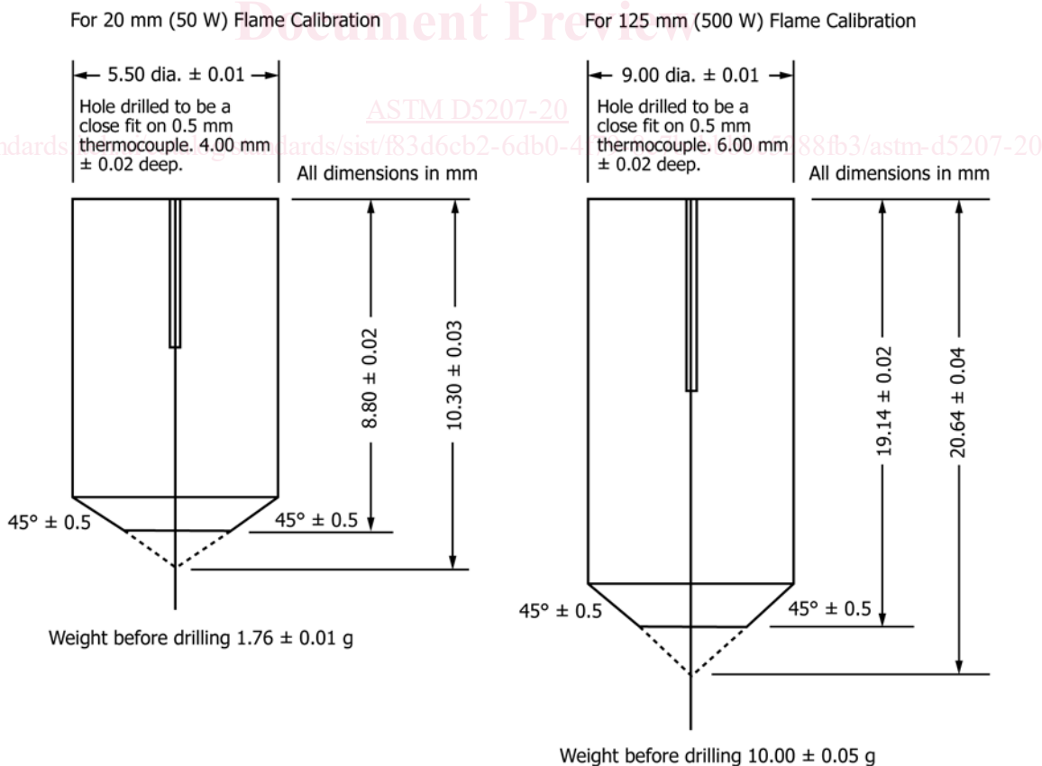
FIG. 1 Copper Slug for Thermal Sensor
