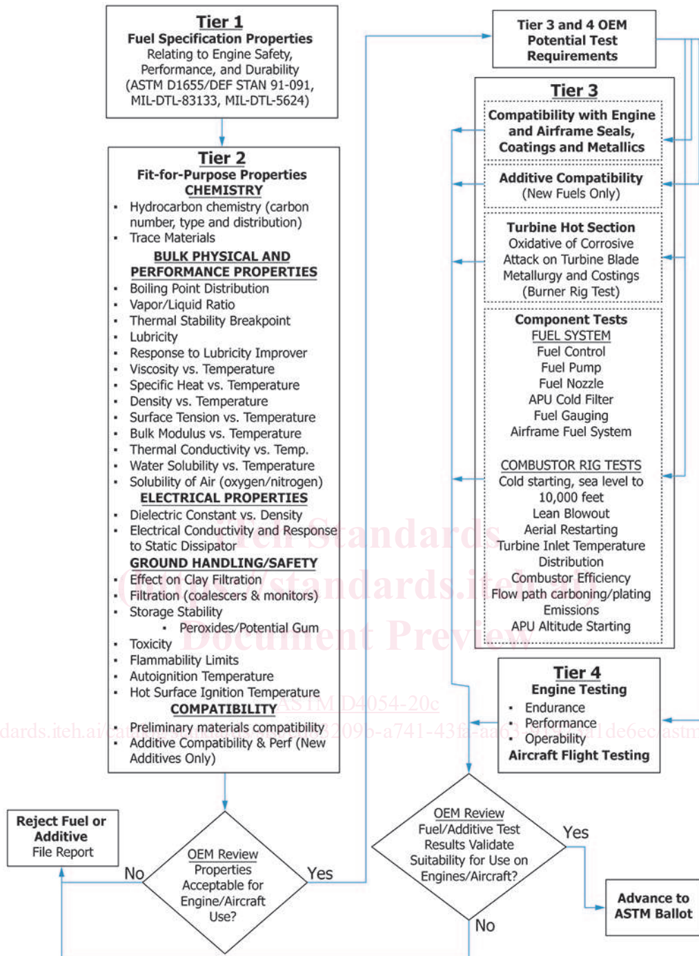
FIG. 2 Test Program
