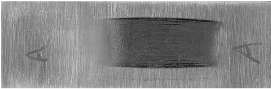
FIG. 5 Typical Uniform Wear Scar
