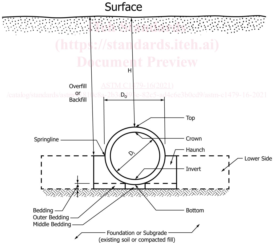
FIG. 1 Pipe/Installation Terminology
