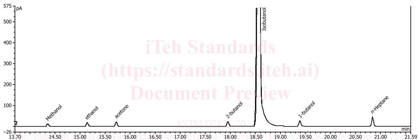
FIG. 2 Sample Chromatogram (1 % Impurities in isobutanol)
