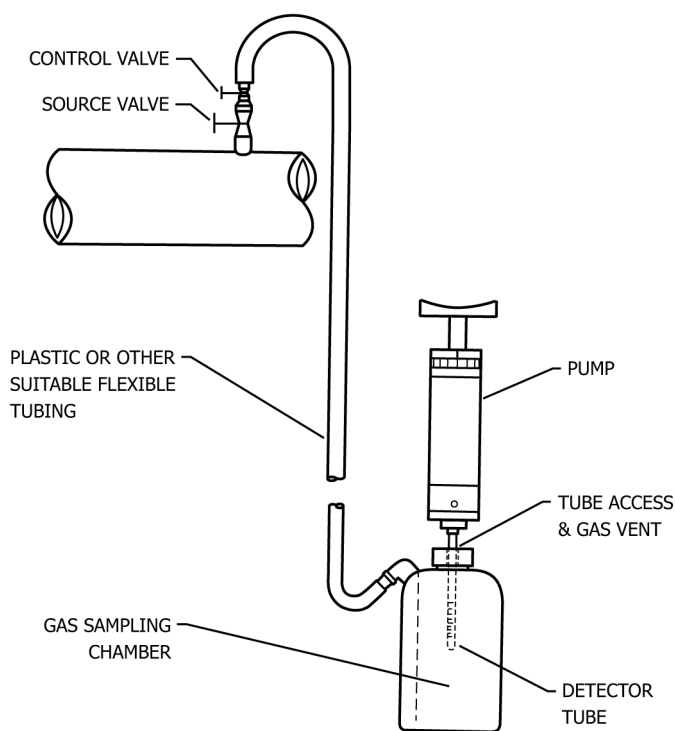
FIG. 1 Apparatus Schematic
