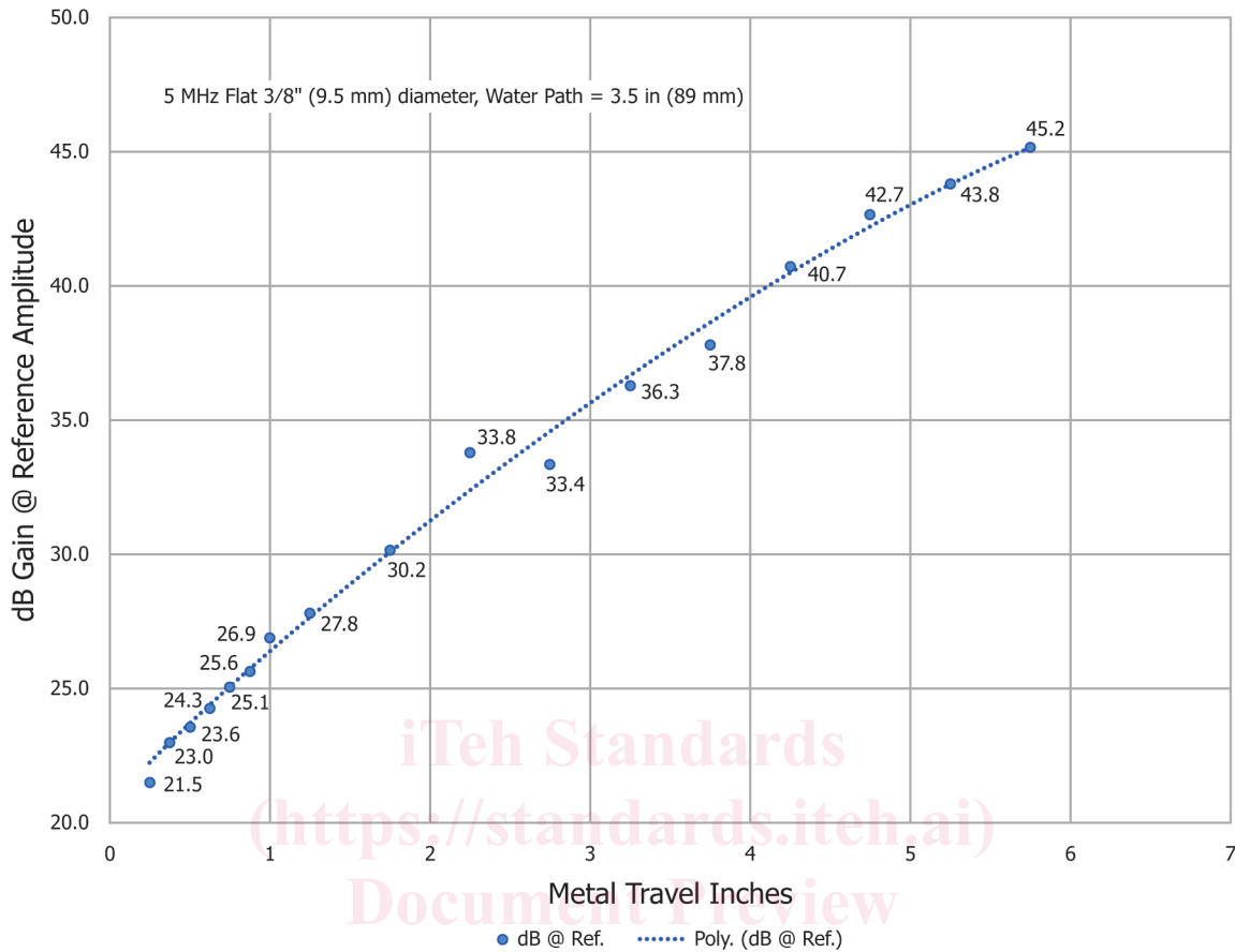
FIG. 4 Distance Amplitude Response Plot
