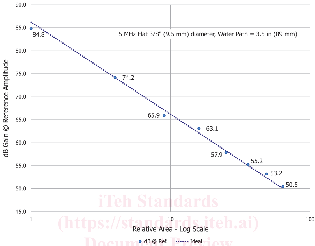
FIG. 3 Area Amplitude Response Plot
