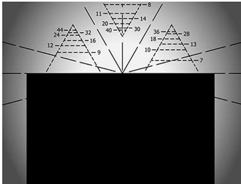
FIG. 2 Shadow-Graph (20x Magnification) of 1/64 in. (6.4 mm) Diameter Flat-Bottom Hole Replica as Viewed on 62.5x Optical Comparator with Commercial Viewing Screen (Reduced 1/2)
