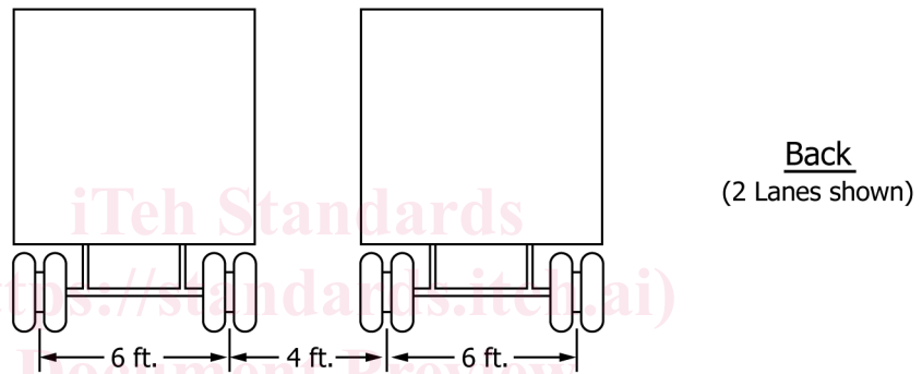
FIG. 1 Loading Arrangements (AASHTO HL-93)
