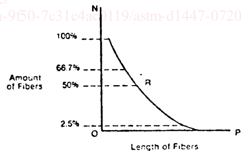
FIG. 3 Diagram Showing Digital Fibrograph Length Measurements
