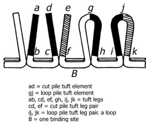
FIG. 1 Cross-Section of Tufted Pile Yarn Floor Covering
