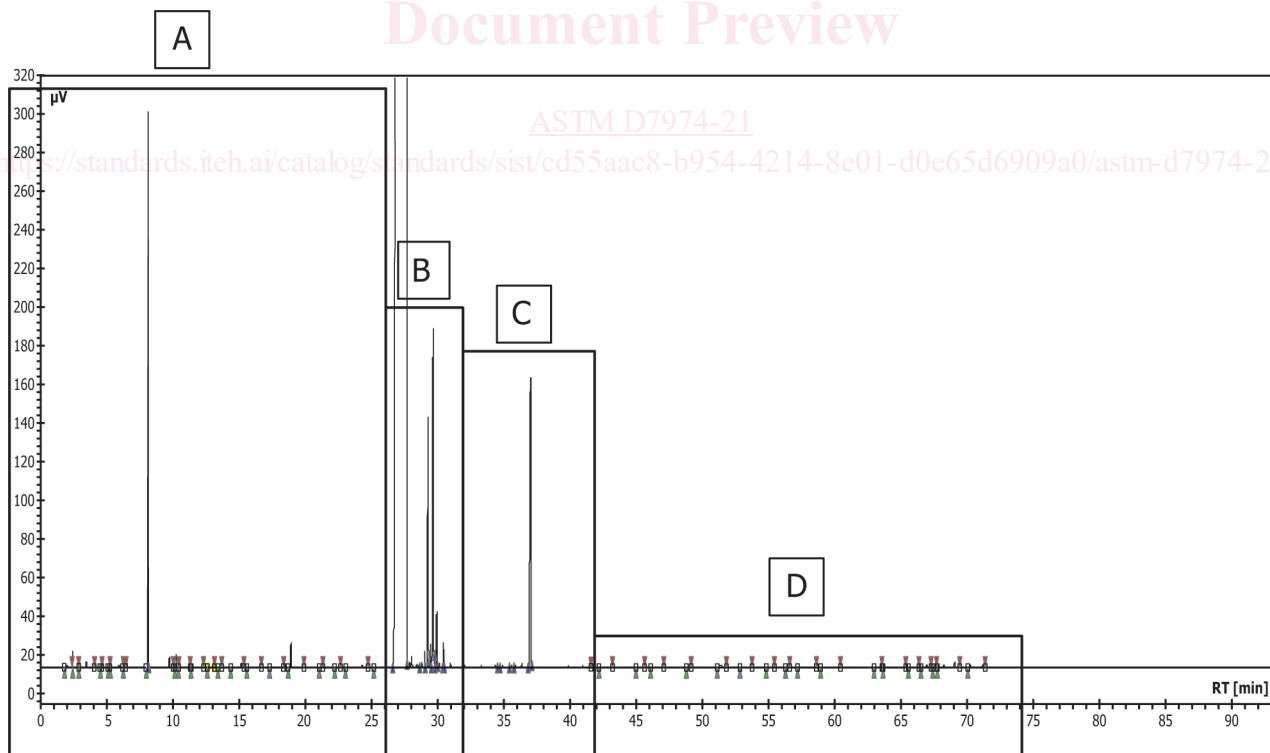
FIG. 1 Chromatogram of a Reference Distilled Farnesane
