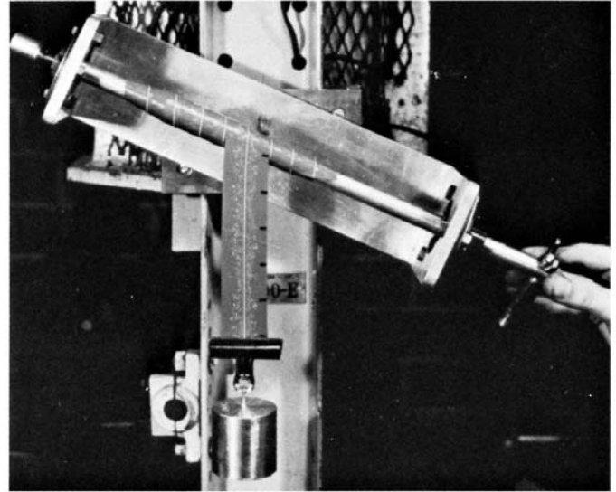
FIG. 1 Inclined Mandrel Tack Test Fixture
