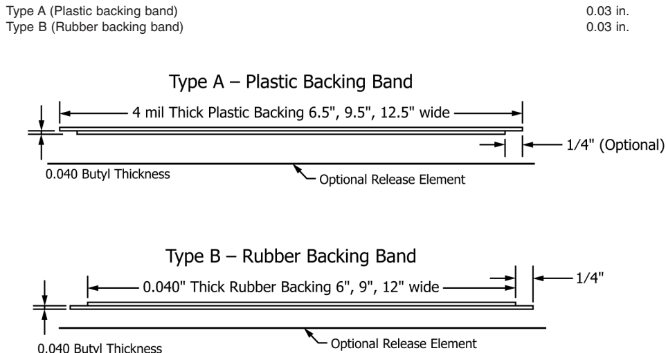
FIG. 3 Sealing Band Type III (Not to Scale)
