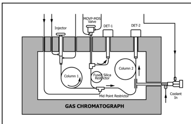
FIG. 4 Heart-Cut Operation
