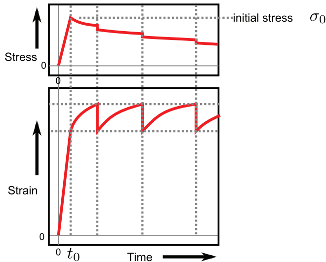
FIG. 2 Derivation of Stress-Relaxation Curve from Continuous Relaxation Stress-Relaxation Technique
