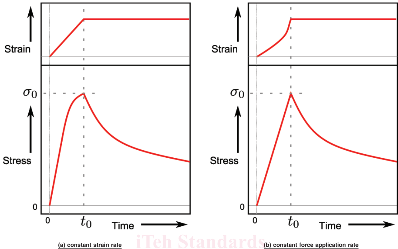
FIG. 1 Characteristic Behavior During Force Application—Force-Application Period in a Relaxation Stress-Relaxation Test—(a)
