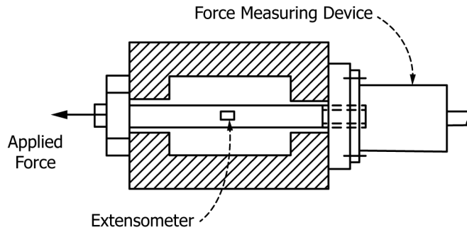
FIG. 34 Tension Stress-Relaxation Test Using Periodic Force Measurement
