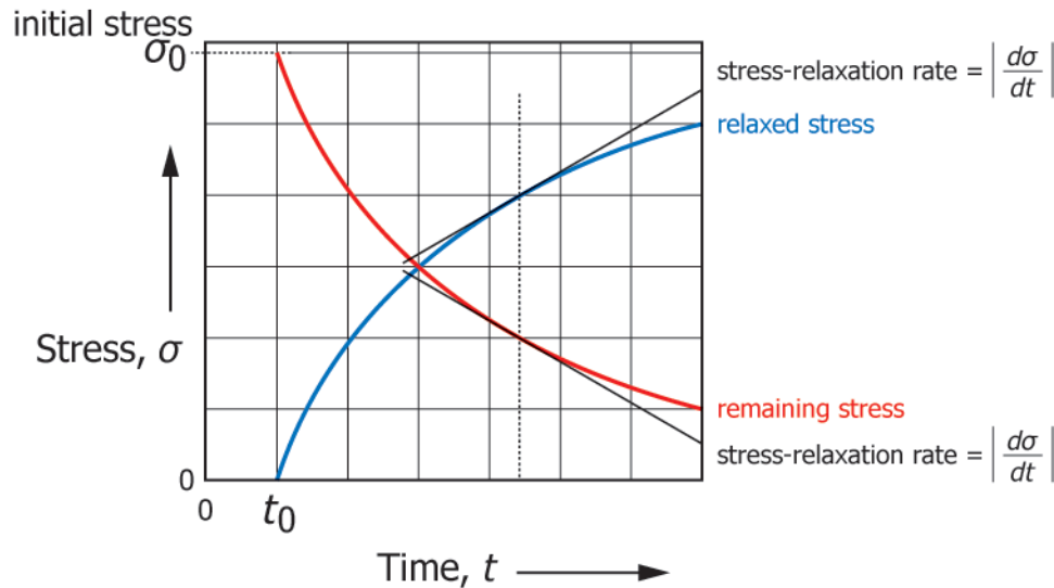
FIG. 13 - Characteristic Behavior During Force Application Period in a Relaxation Test (b) Typical Stress-relaxation Curve (continued)
