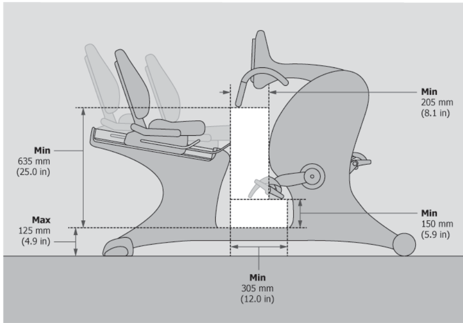
FIG. 6 Dimensions for Transition Area Box
