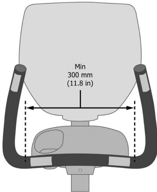
FIG. 9 Handlebar Length
