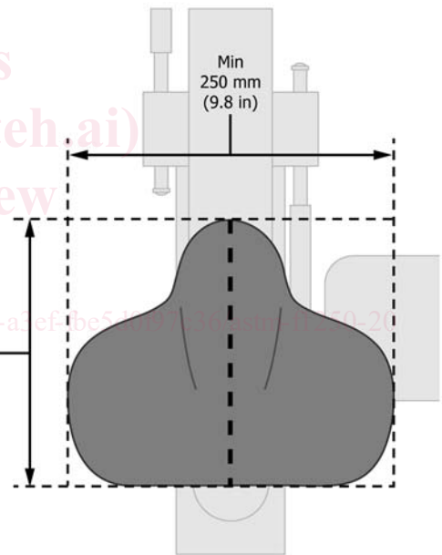
FIG. 8 Upright Exercise Bicycle Seat Width and Depth
