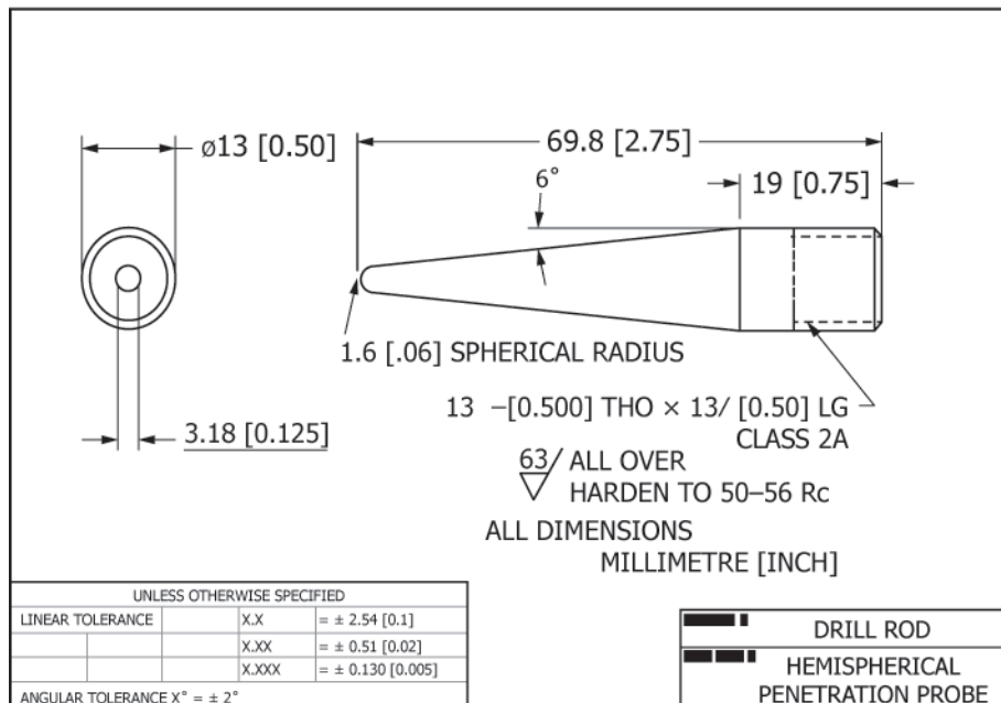
FIG. 1 Penetration Probe
