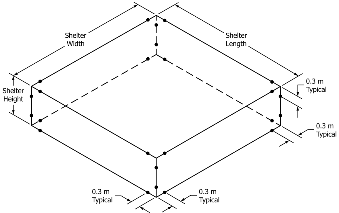
FIG. 5 Corner Test Point Assignment
