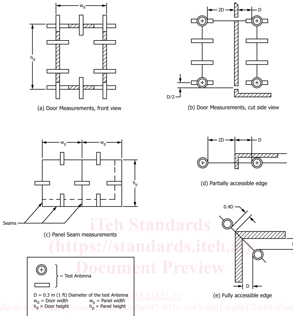
FIG. 7 Door, Seam, and Edge Measurements for Magnetic Field
