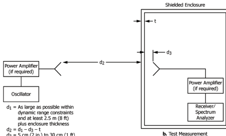
FIG. 2 Plane Wave Field Test Procedures
