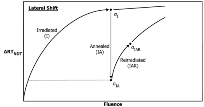
FIG. X2.1 Lateral Shift Method for Estimating Reirradiation Embrittlement
