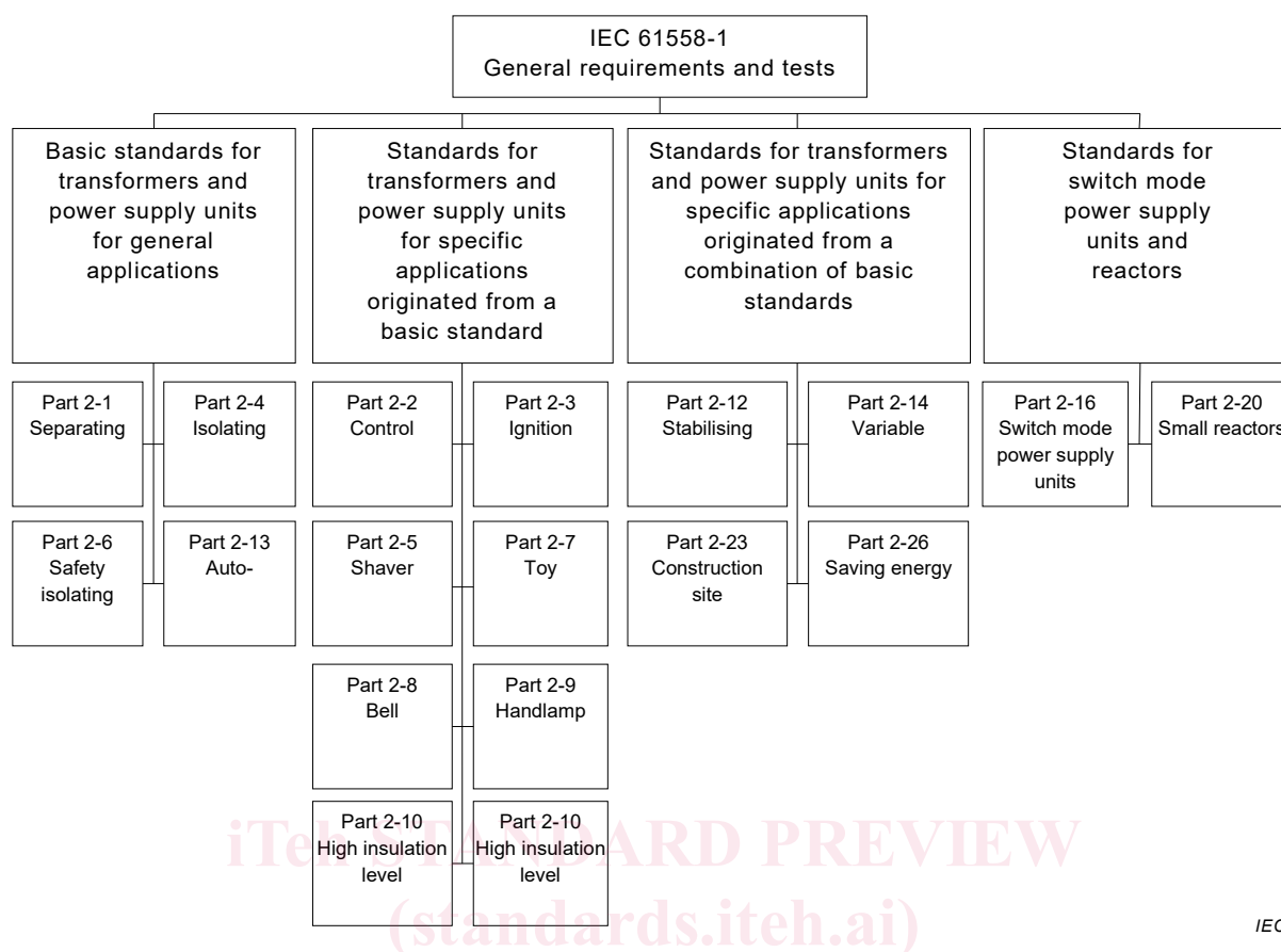
Figure 1 – IEC 61558 principle
