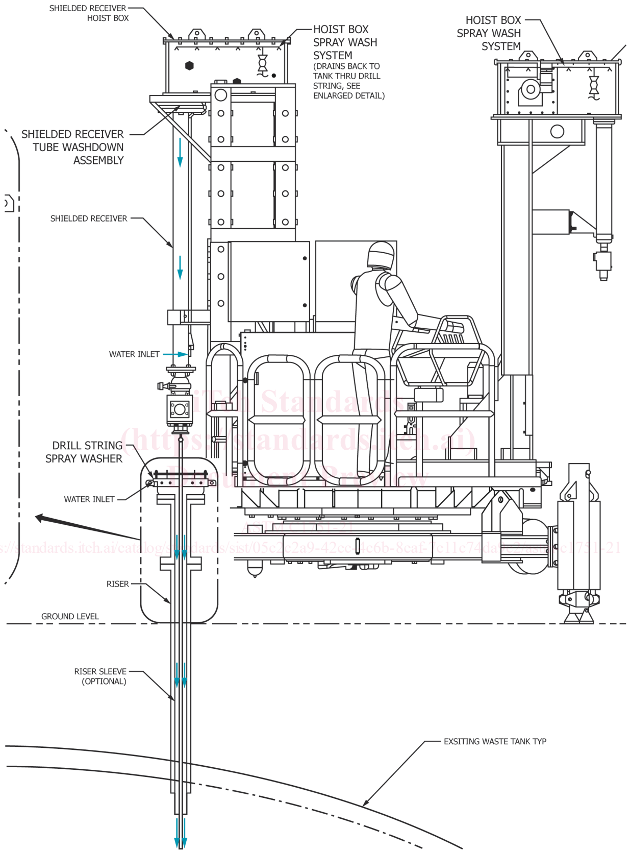
FIG. 4 b. Core Sampling Platform (continued)
