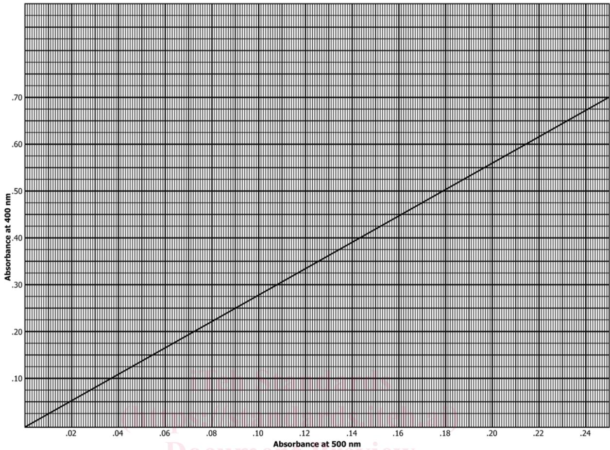
FIG. 1 Correction Graph
