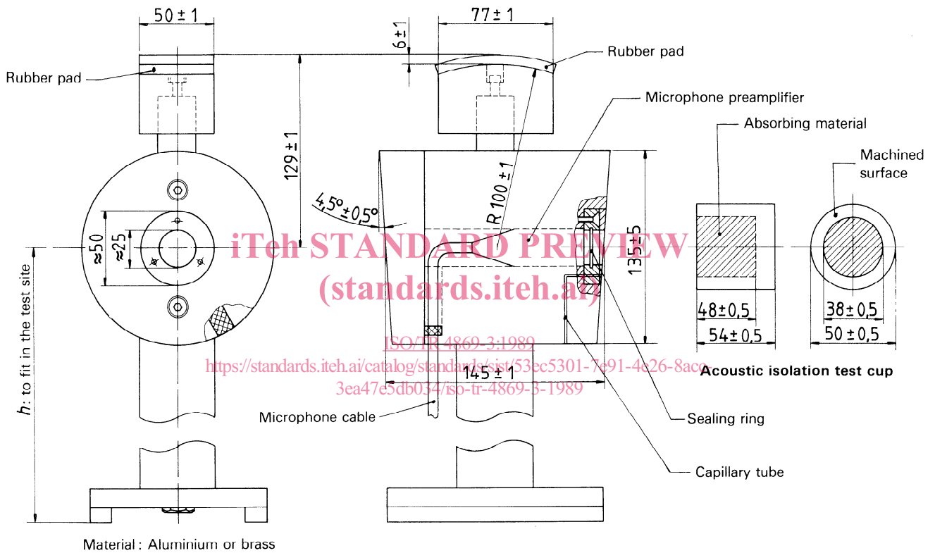
Figure 1 – Example of an acoustic test fixture
