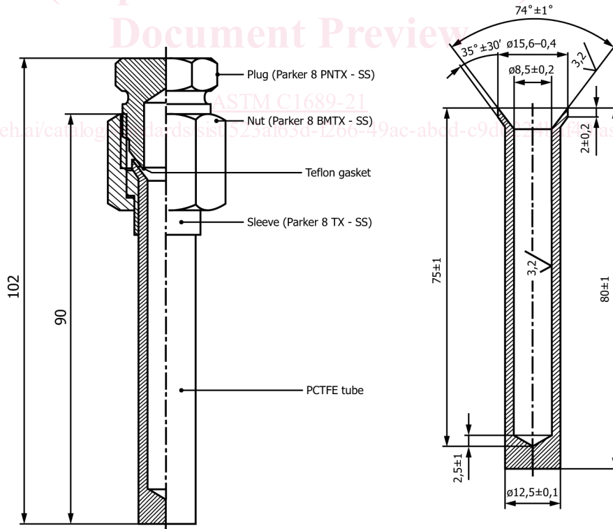
FIG. 4 Example of Polychlorotrifluoroethylene Subsample Tube
