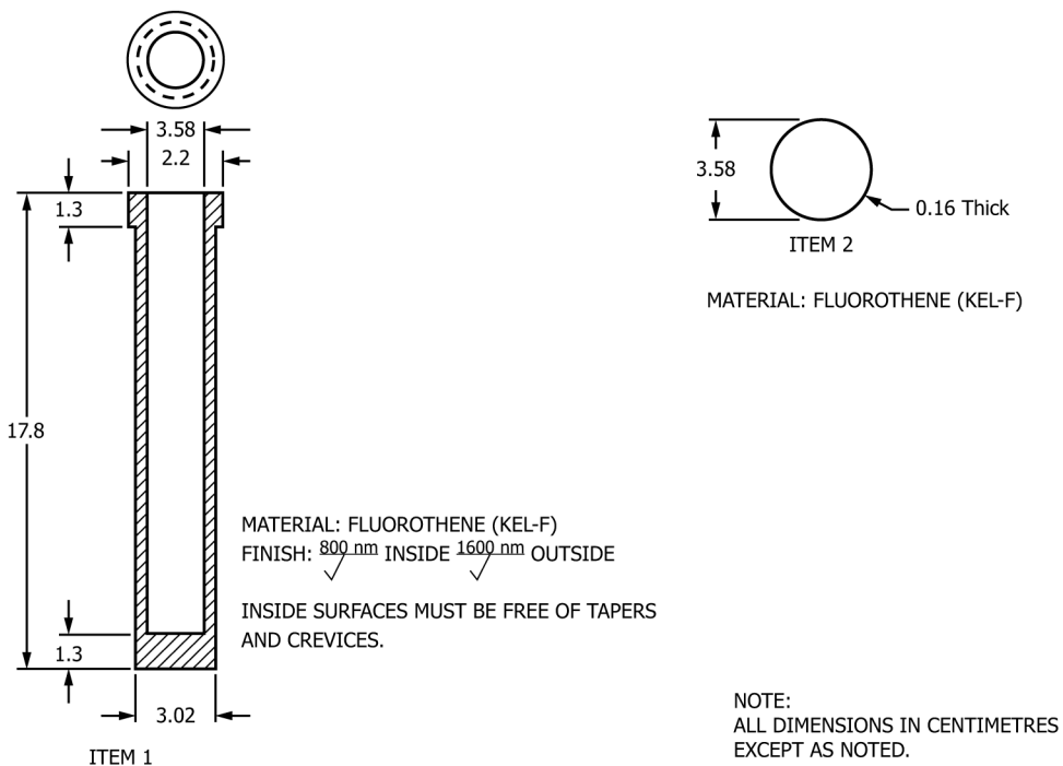
FIG. 5 Example of Polychlorotrifluoroethylene Knock-out Tube
