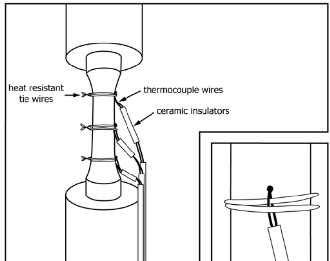
FIG. 1 Installation with Welded Junctions (Inset: Attachment Detail)
