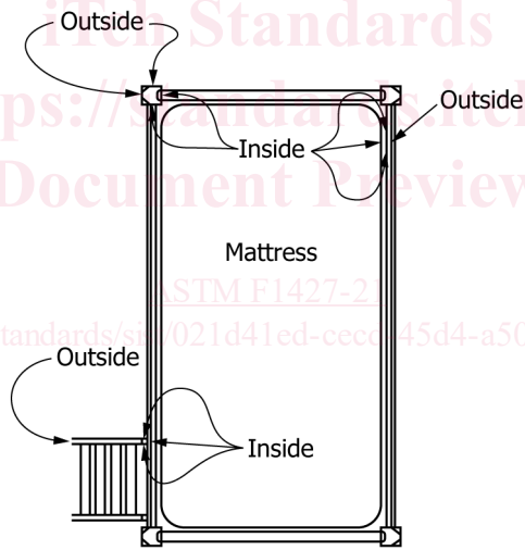
FIG. 3 Vertical Protrusions
