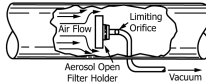
FIG. 5 Faulty Sample from a Rapid-Ducted Gas Stream
