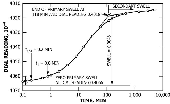
FIG. 1 Time-Swell Curve
