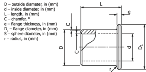
FIG. 2 Standard Flange Bearing
