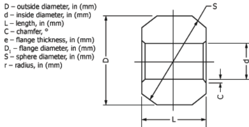
FIG. 4 Standard Spherical Bearing
