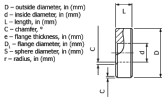
FIG. 3 Standard Thrust Bearing
